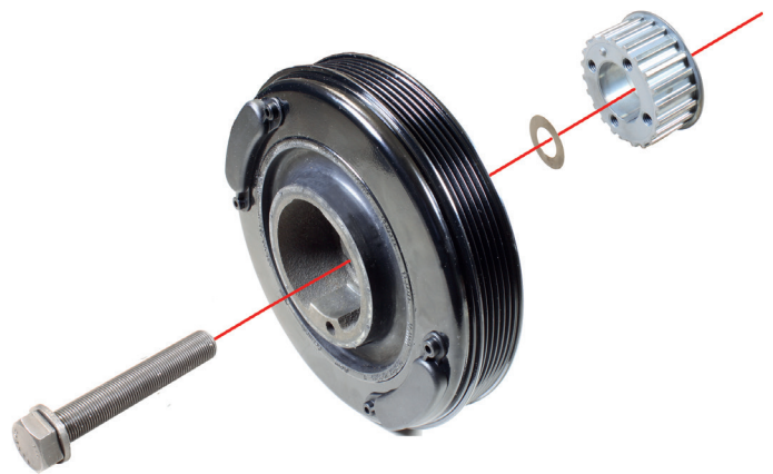
The belt pulley set 544 0002 20 comprises a crankshaft vibration damper with main crankshaft bolt and diamond-encrusted washer.
